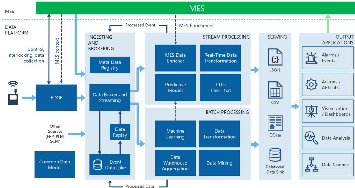
Figure 1 IoT Data Platform architecture
