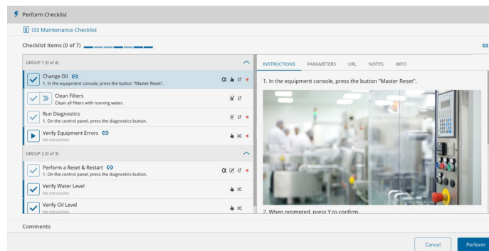
Figure 2 Checklist example
